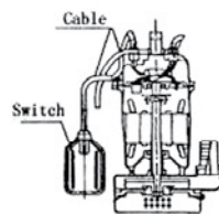
Sketch drawing of Key switch attached to drainage pump
