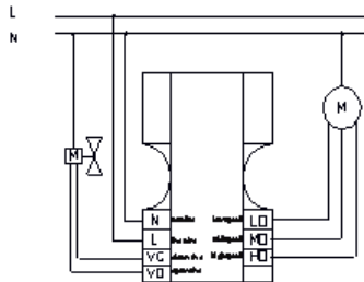
Wiring method of controlling double wire valve
