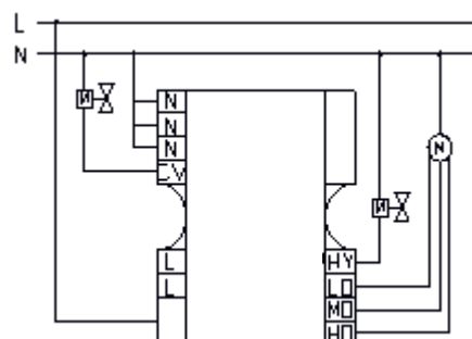
Wiring diagram of electromotion draught of thermostat
