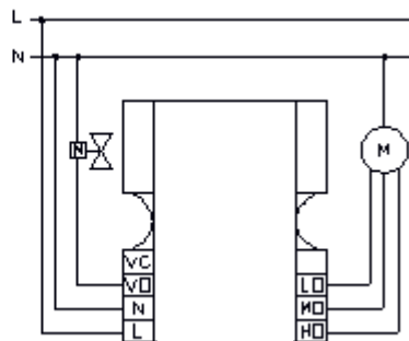
Method of controlling double wire valve
