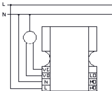
Method of quadruple pipe wiring
