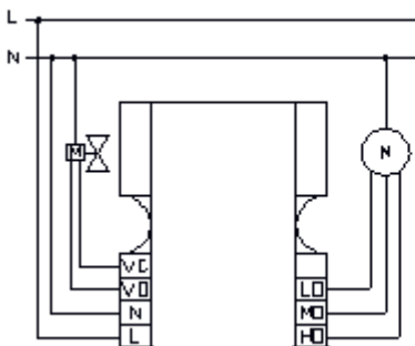
Method of controlling triple wire valve
