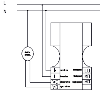
Wiring diagram of electromotion draught of thermostat
