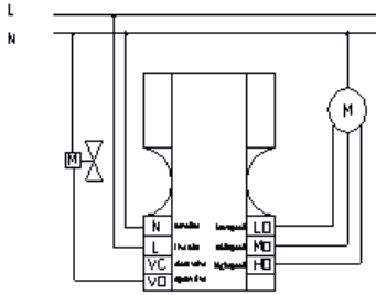
Method of controlling triple wire valve.
