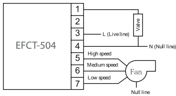
EFCT-504 Cooling/heating 2 or 4-pipe system
